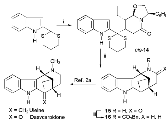
Scheme 4 Reagents and conditions: (i) n -BuLi, THF, –78 °C, then 7 . (ii) Na, liq. NH 3 , –33 °C, then TiCl 4 , CH 2 Cl 2 , 25 °C. (iii) BH 3 ·Me 2 S, toluene, reflux, then ClCO 2 Bn, K 2 CO 3 .
