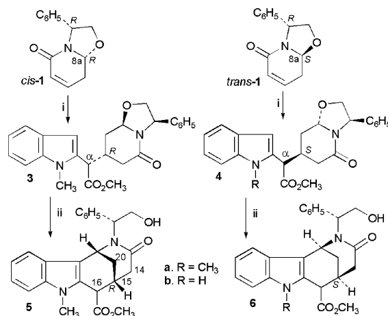
Scheme 1 Reagents and conditions: (i) 2a or 2b , LDA, THF, -78^\circ\text{C} , then 1, 0^\circ\text{C} . (ii) TiCl 4 , CH 2 Cl 2 , rt (reflux from 3 ).
