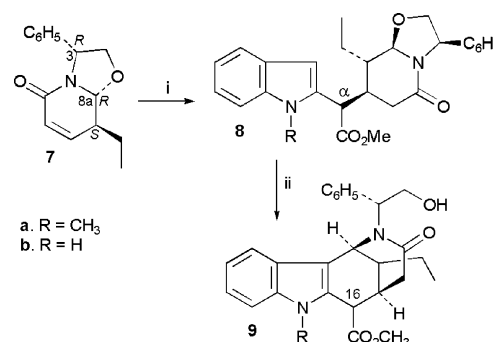
Scheme 2 Reagents and conditions: (i) 2a or 2b , LDA, THF, -78^\circ\text{C} , then 7 , HMPA, CuCN (from 2b ), rt. (ii) TiCl 4 , CH 2 Cl 2 , reflux.
