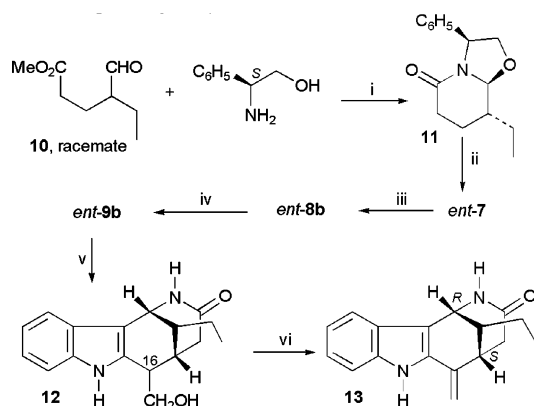
Scheme 3 Reagents and conditions: (i) Et 2 O, anh. Na 2 SO 4 , 0 °C, 1 h, then 70 °C, 10–15 mm Hg. (ii) C 6 H 5 S(O)OMe, KH, THF, reflux, then toluene, Na 2 CO 3 , reflux. (iii) 2b , LDA, THF, –78 °C, then ent - 7 , HMPA, CuCN, rt. (iv) TiCl 4 , CH 2 Cl 2 , reflux. (v) Na, liq NH 3 , –33 °C. (vi) MsCl, Et 3 N, CH 2 Cl 2 , 0 °C, then DBU, THF, reflux.
